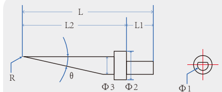
Single-Cut Stylus
