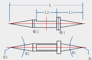
Double-Directional Stylus
