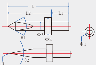
Double-Cut Stylus
